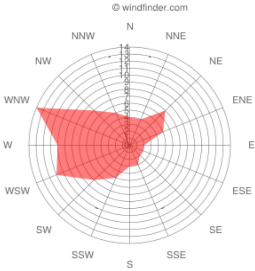
Wind dir. distribution Zürich-Kloten July
